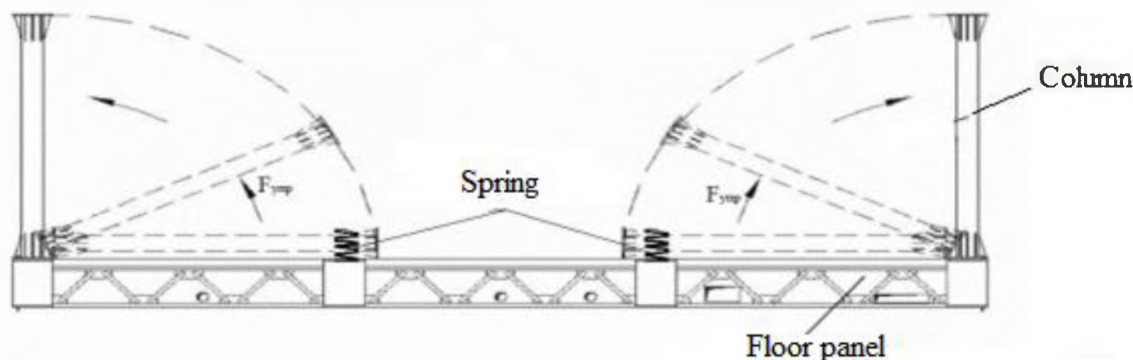
Fig. 3. The mechanism of using a spring to speed up the installation of columns
