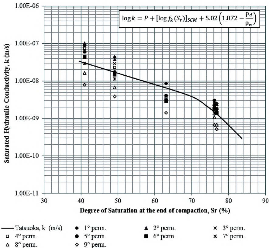
Fig. 8. Comparison between the experimental k values (808I soil) and the Tatsuoka's model (Giusti 2017)
