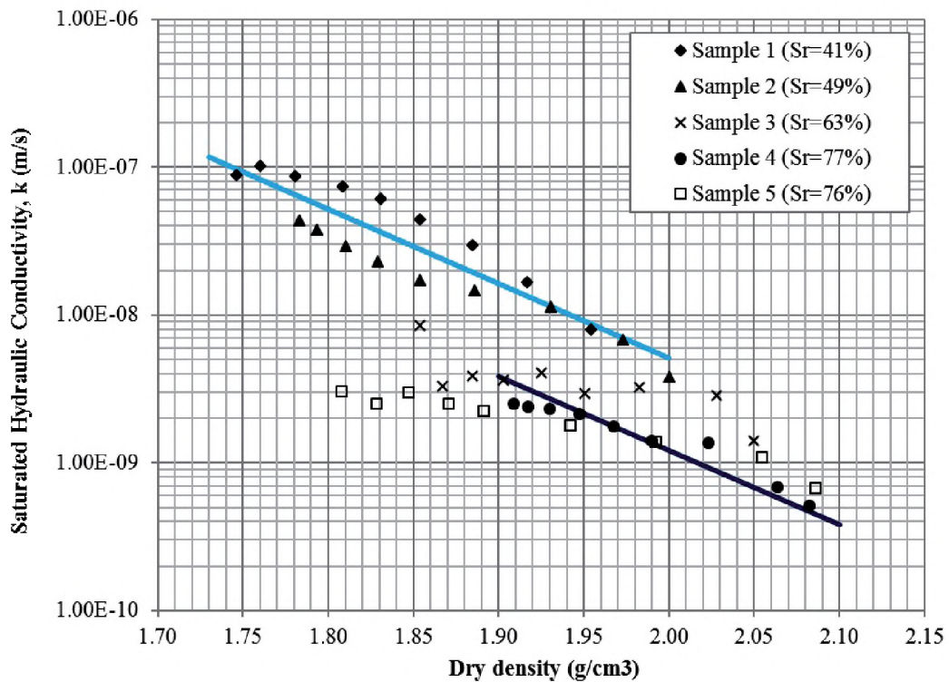
Fig. 5b. Dependence of k on the initial degree of saturation and dry density for 808I soil (Giusti 2017 [13] — data)
