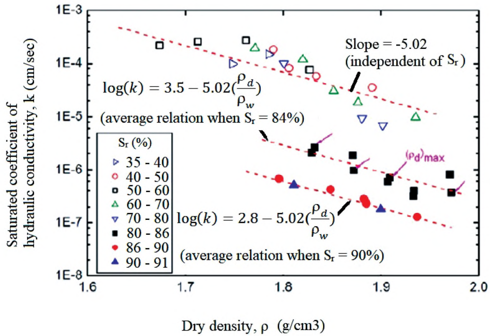
Fig. 5a. Dependence of k on the Saturation degree and Dry density (Tatsuoka 2015) [21]
