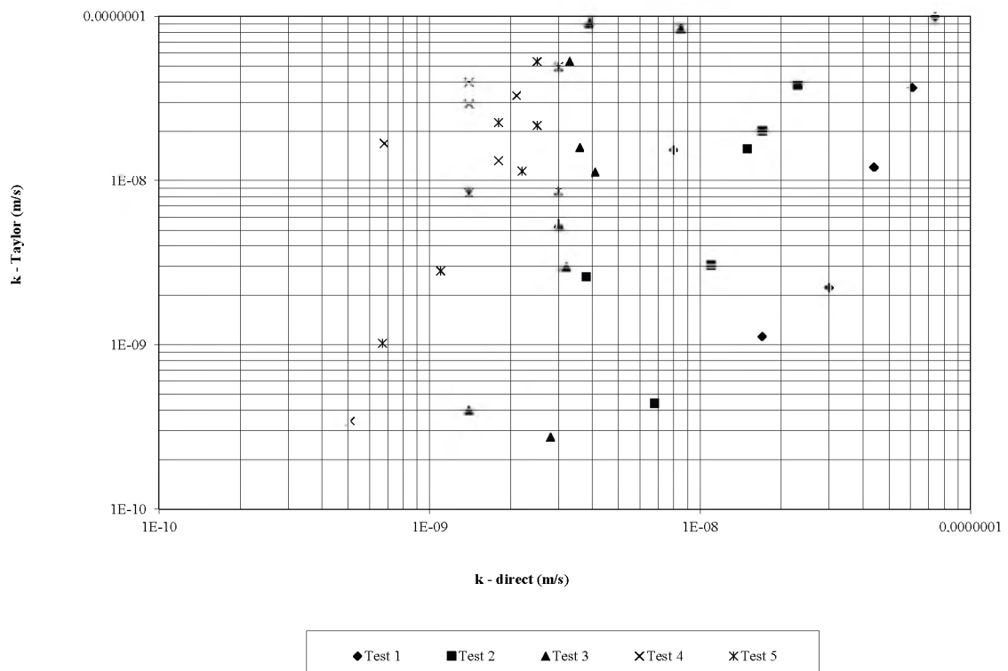
Fig. 9b. Comparison of k values from direct measurement and Taylor (1948) method (808I soil)
